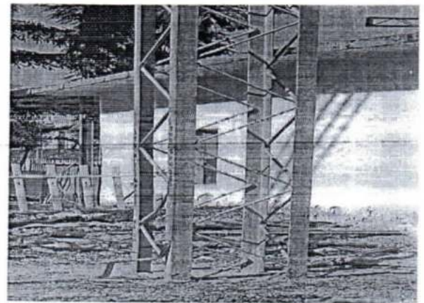
FIG.3 LACING SYSTEM
