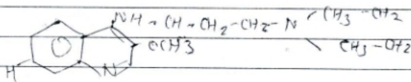
Quinacrine.
