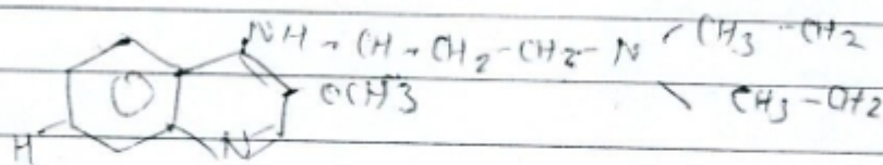
Quinacrine.
