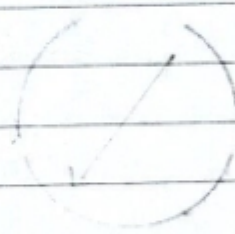
Plane polarised light.
